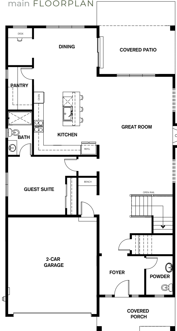
main FLOORPLAN
