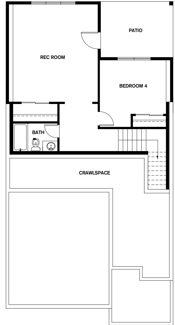
lower FLOORPLAN
