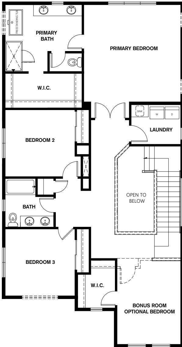
upper FLOORPLAN
