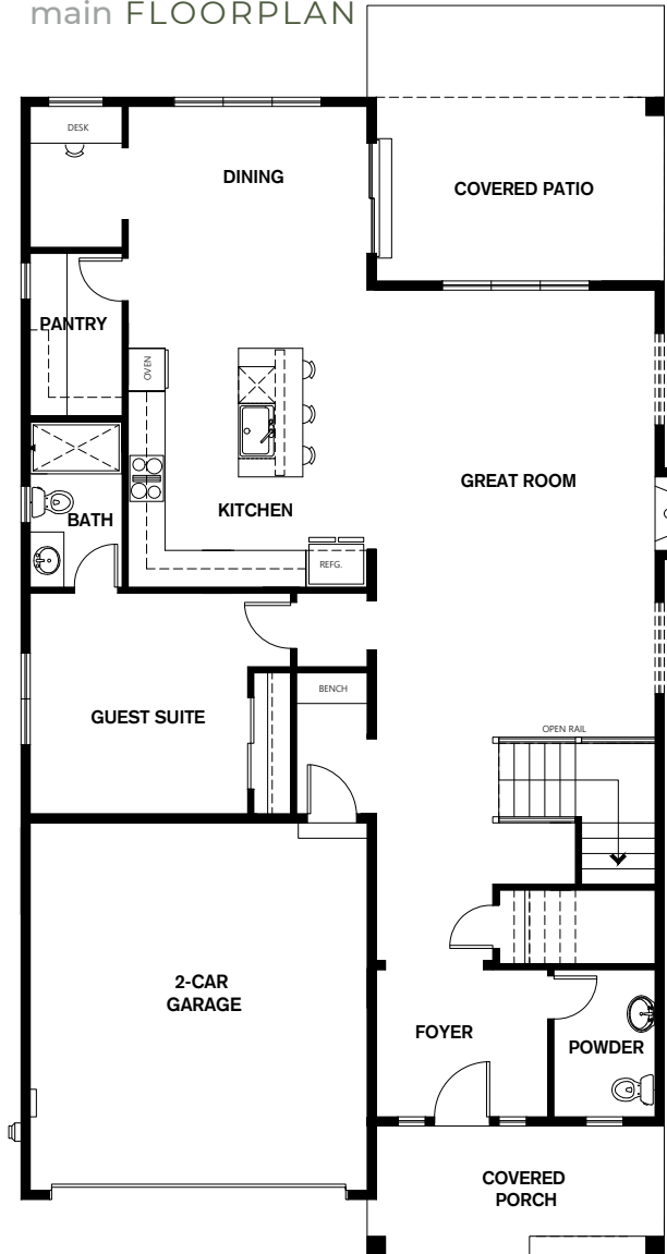
main FLOORPLAN
